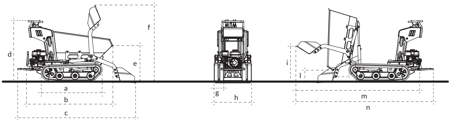
DIMENSIONS (mm)
